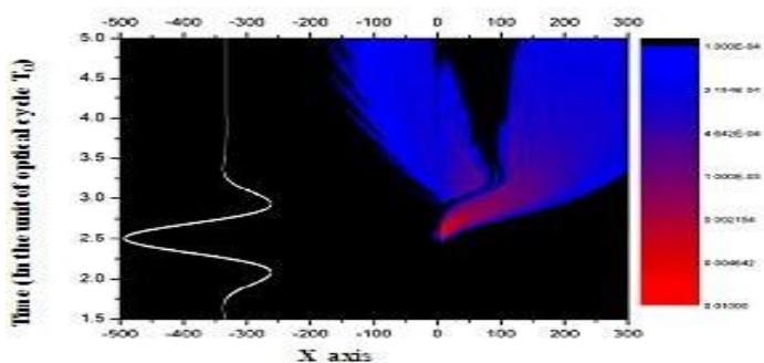
Figure 3: Wavepacket evolution of ionized electrons, with the white line standing for FEL.
