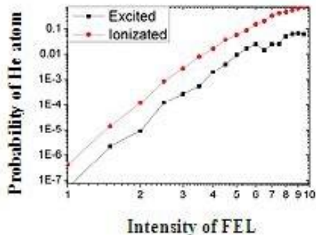
Figure 1: The probability of He atom's ionization and excitation changes with the intensity of FEL in unit of 1014W/cm^2 .
