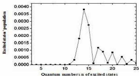
Figure 2: Population of different excited states of He atom irradiated by FEL.
